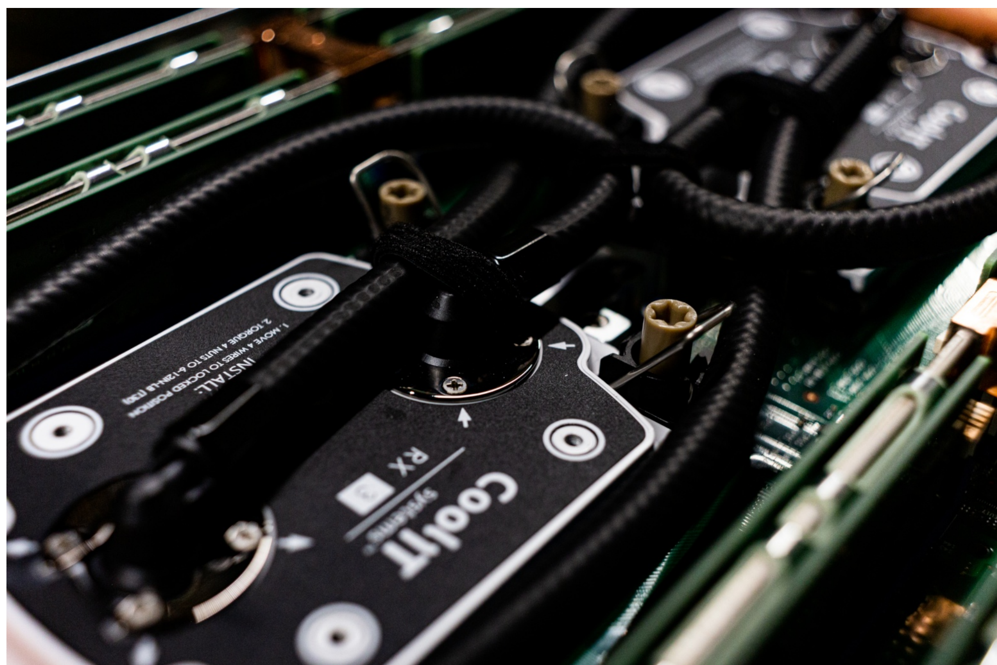
Inside view of one of the almost 1000 water-cooled compute nodes in the "Fritz" supercomputer at NHR@FAU
